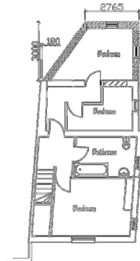
Proposed First Floor
