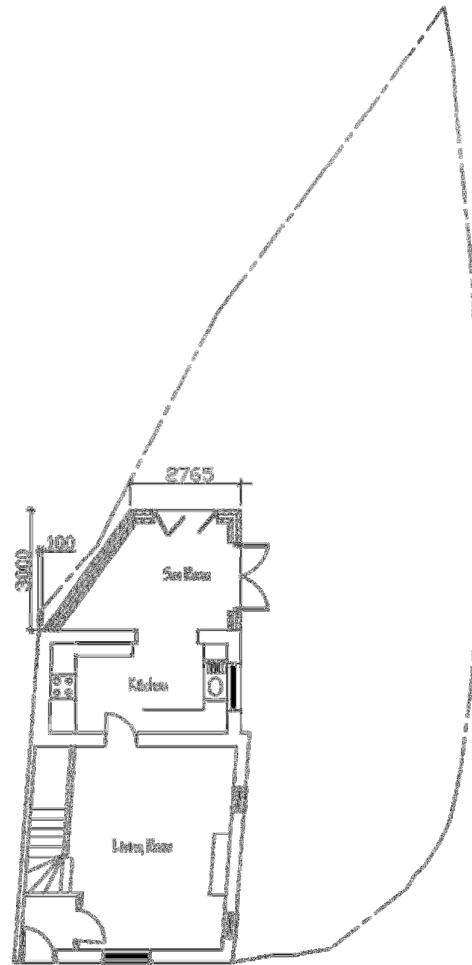
Proposed Site Layout 1:200
