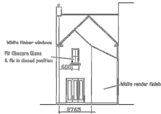
Proposed Rear
